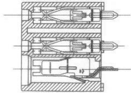
SEC. B-B
